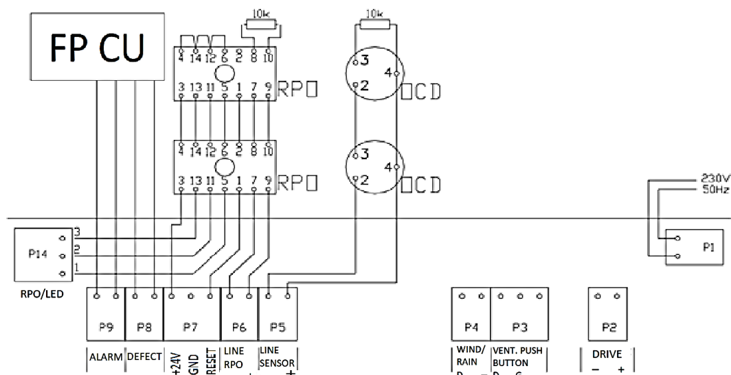
Fig. 4 Alternative connection diagram with mcr RPO-1 emergency pushbuttons and optical smoke sensors.
