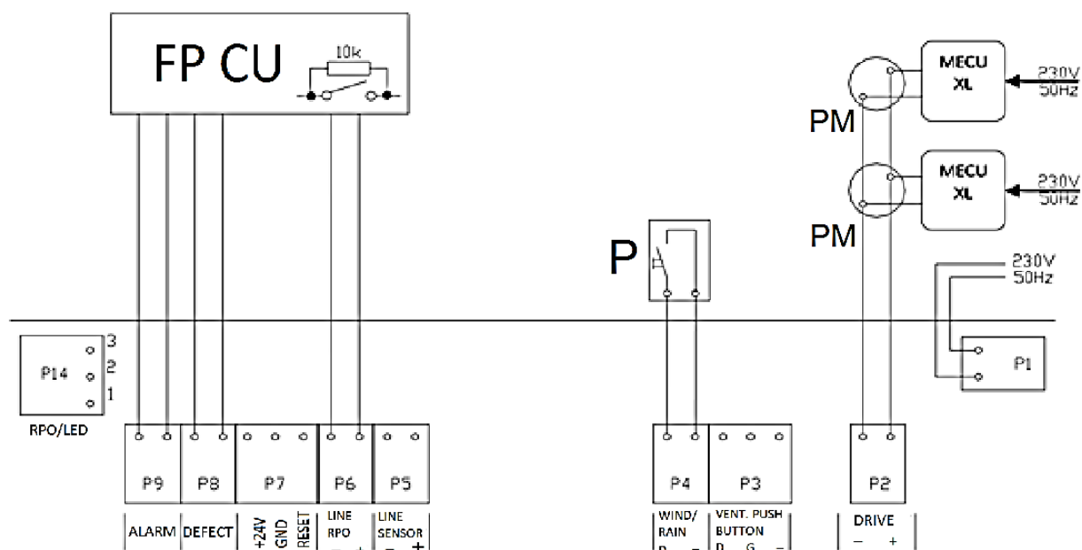
Fig. 3 Typical configuration of smoke exhaust system with mcr 0204 unit.
